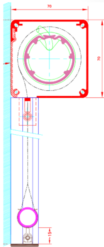
Coulisse 25/17
