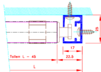
Coulisse 25/17
